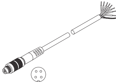
CAB-M8-4P-fm-co-straight; Xm-PUR; open ends
