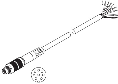
CAB-M12-8P-co-fm-straight; Xm-PUR; open ends
