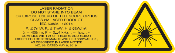
Fig. 2 Laser warning sign and laser label, scanCONTROL 29xx/10BL
