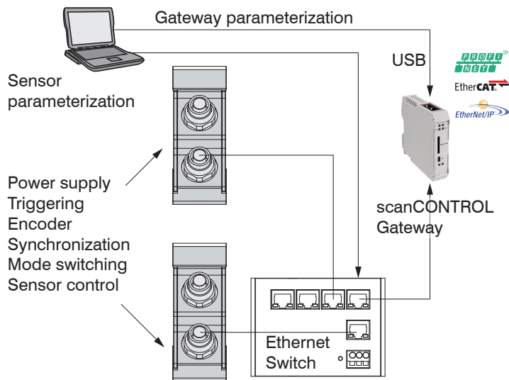
Fig. 36 Network layout for using scanCONTROL Gateway
