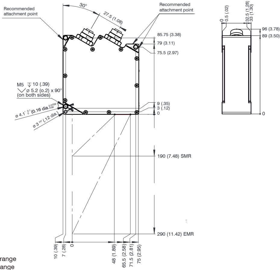
Fig. 14 Dimensional drawing scanCONTROL 29xx-100 sensor, dimensions in mm (inches), not to scale
