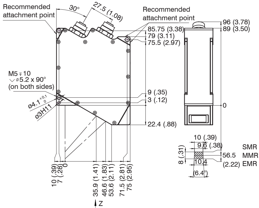
Fig. 11 Dimensional drawing scanCONTROL 29xx-10/BL sensor, dimensions in mm (inches), not to scale
