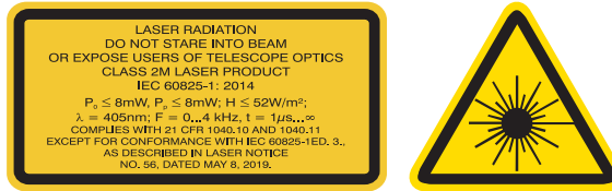
Fig. 3 Laser warning sign and laser label, scanCONTROL 29xx-25/BL, 29xx-50/BL, 29xx-100/BL
