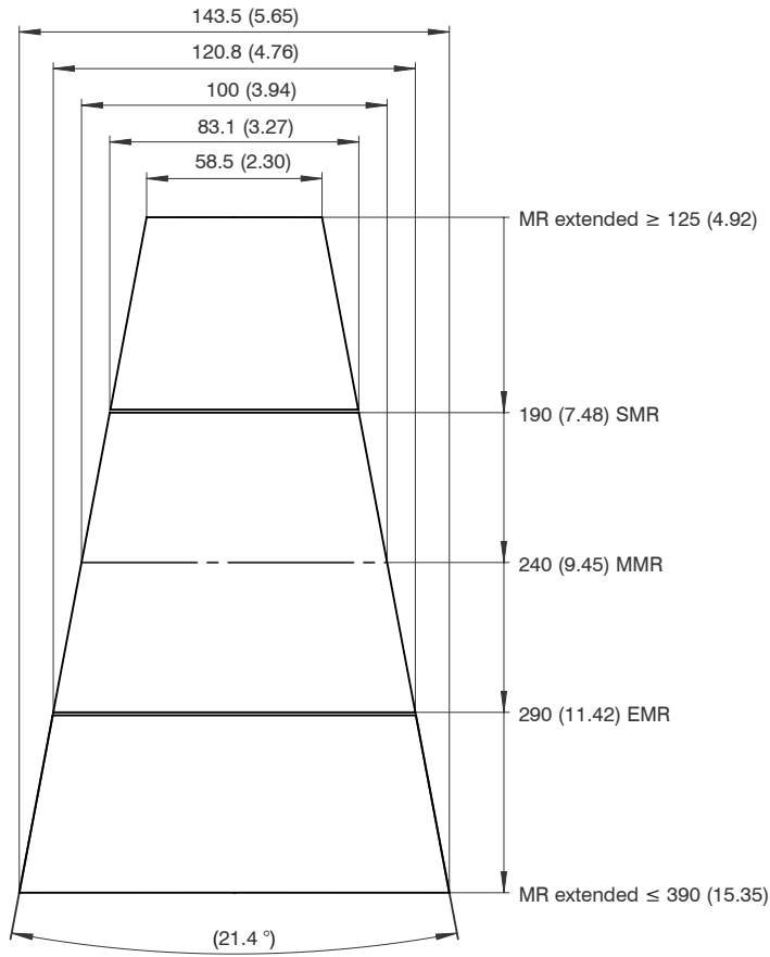
Fig. 15 Measuring field scanCONTROL 29xx-100 sensor, dimensions in mm (inches), not to scale
