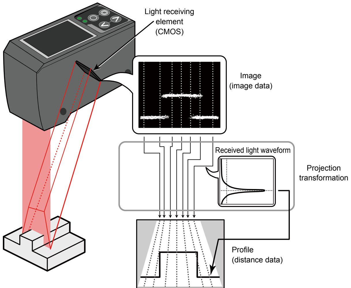
Figure: Schematic diagram of LS series measurement
