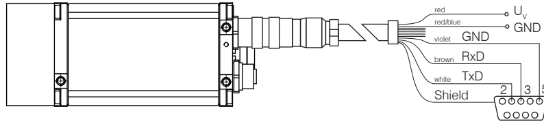
Fig. 13 Wiring RS232 at 9-pole Sub-D female cable connector
