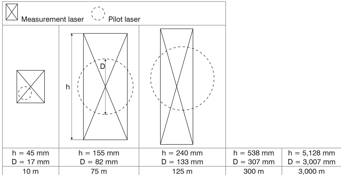
Fig. 8 Tolerance on pilot laser position relative to measurement laser
