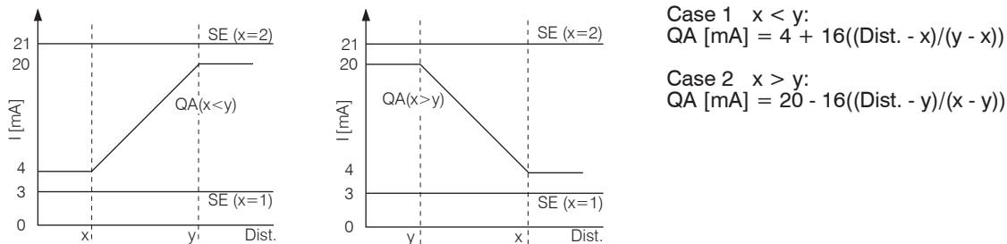
Fig. 12 Signal diagram analog output with x < y and x > y , definition: x \neq y
