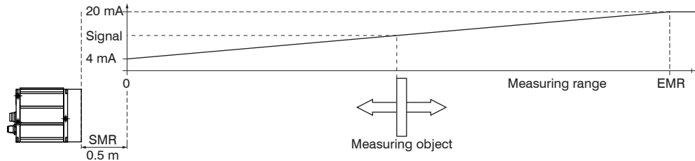
Fig. 7 Start of measuring range and signal characteristic
