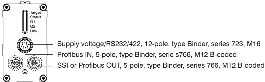
Fig. 9 Connectors on the rear side of the sensor, depends on sensor type
