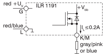
Fig. 15 Wiring switching outputs
