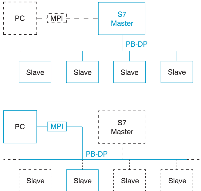
Fig. 18 Slave address
