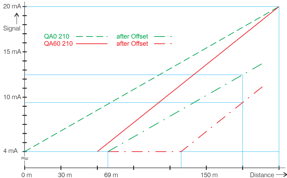
Fig. 20 Analog output with offset displacement at 69 m
